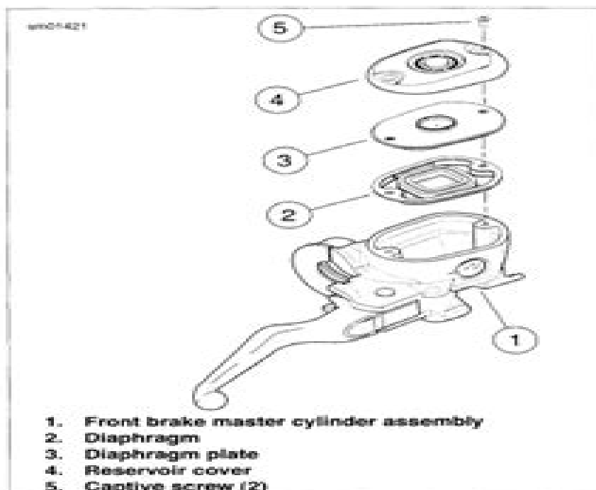
Figure 1-10. Front Brake Master Cylinder Cover Assembly (Typical)
