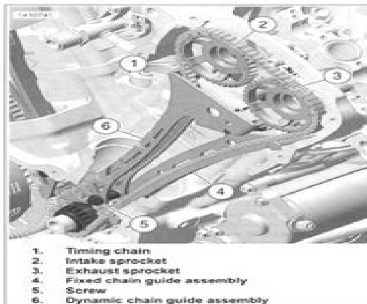
Figure 4-31. Sprockets and Chain (Section view of front cylinder head)
