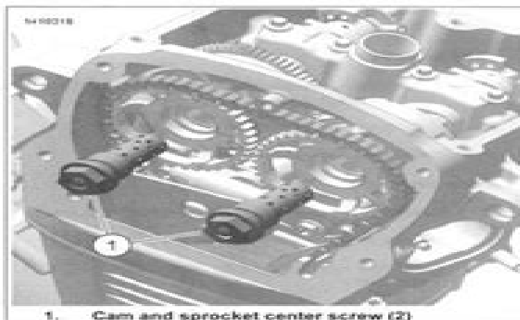
Figure 4-28. Cam and Sprocket Center Screw
