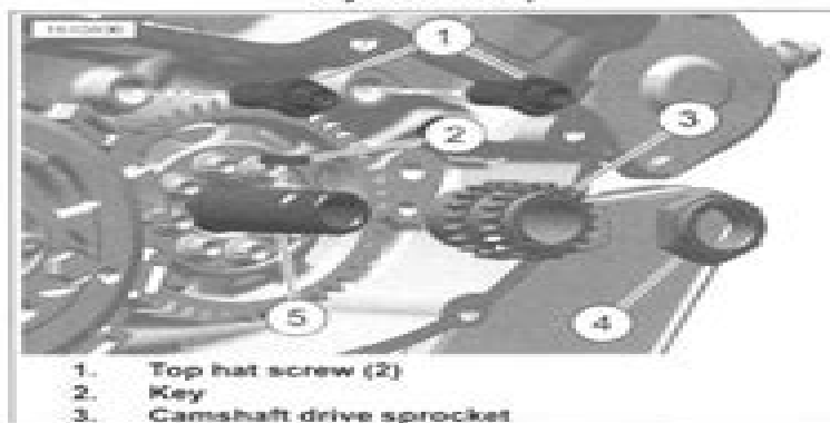
Figure 4-32. Top Hat Screw and Camshaft Drive Sprocket
