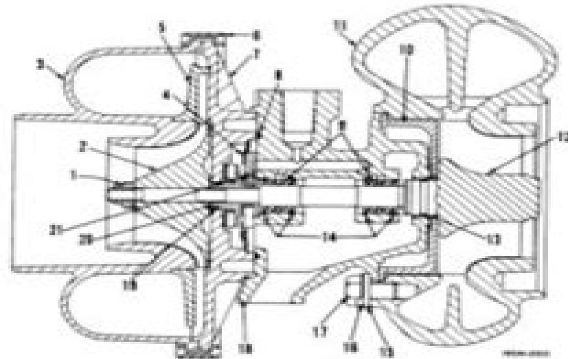
Illustr. 1. Cross section of turbocharger.
