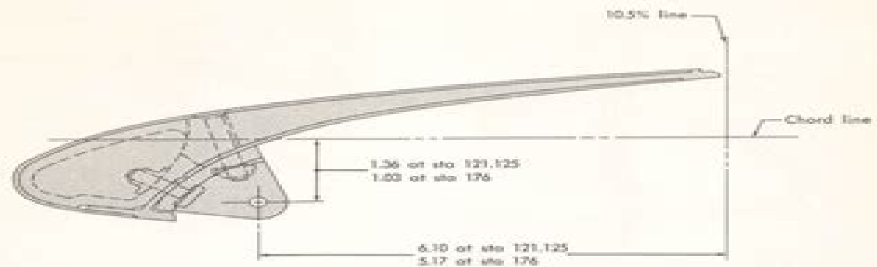
VIEW E SLAT ATTACHMENT FITTING
