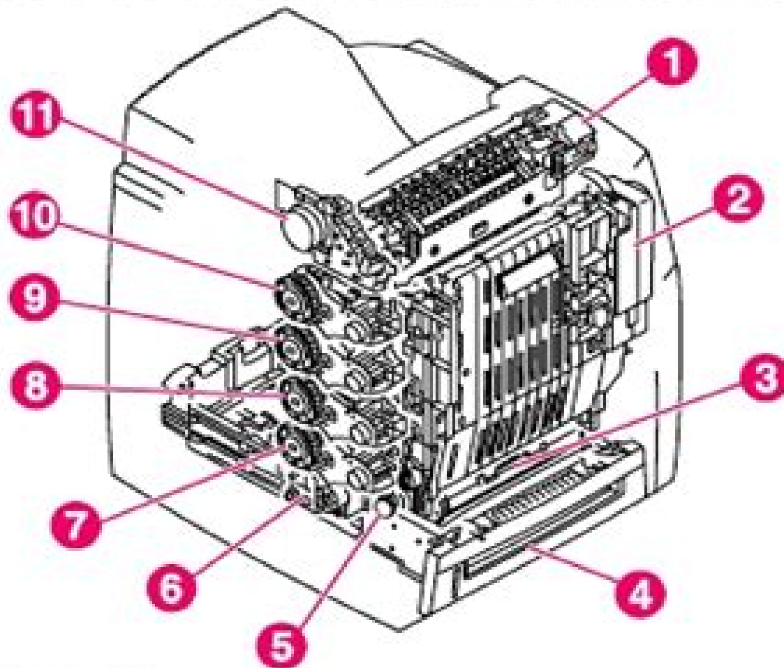
Figure 8-1 Major components of the HP Color LaserJet 4600 Series printer
