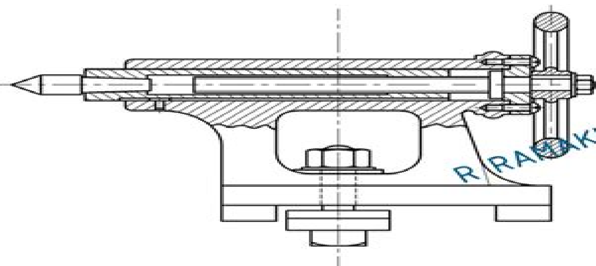
Sectional Elevation
