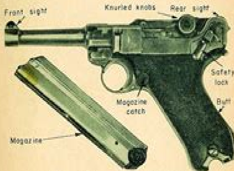
Figure 2.—Luger pistol and magazine.
