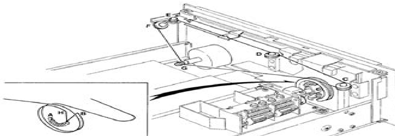
Figure 1. Dial Stringing
