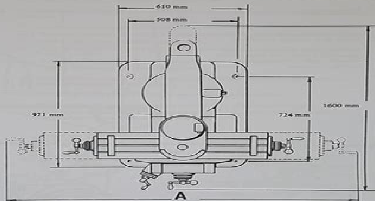
'A' DIMENSION
