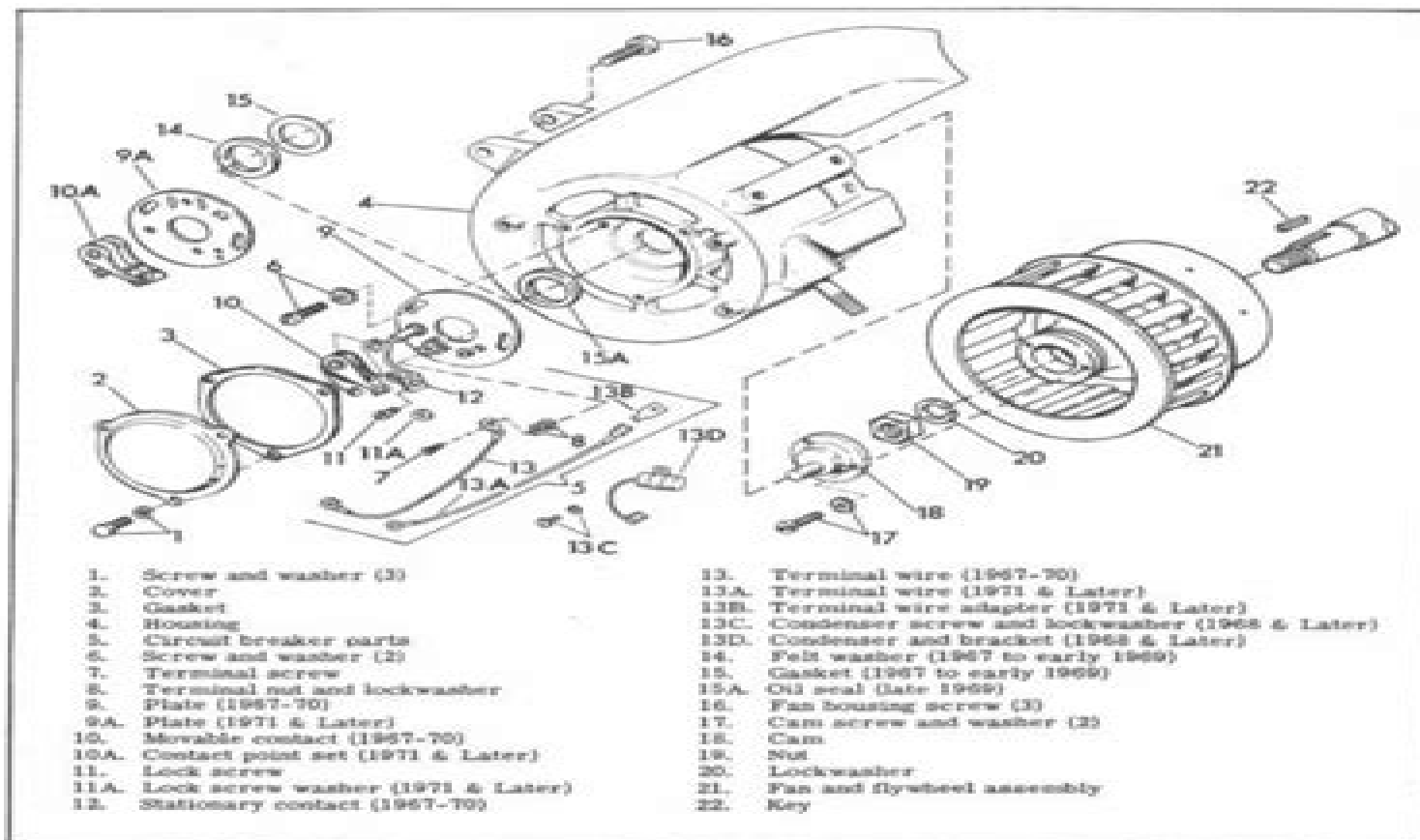
Figure 5F-12A. Circuit Breaker and Fan (1967 & Later D, 1969-1972 DC Models) - Exploded View
