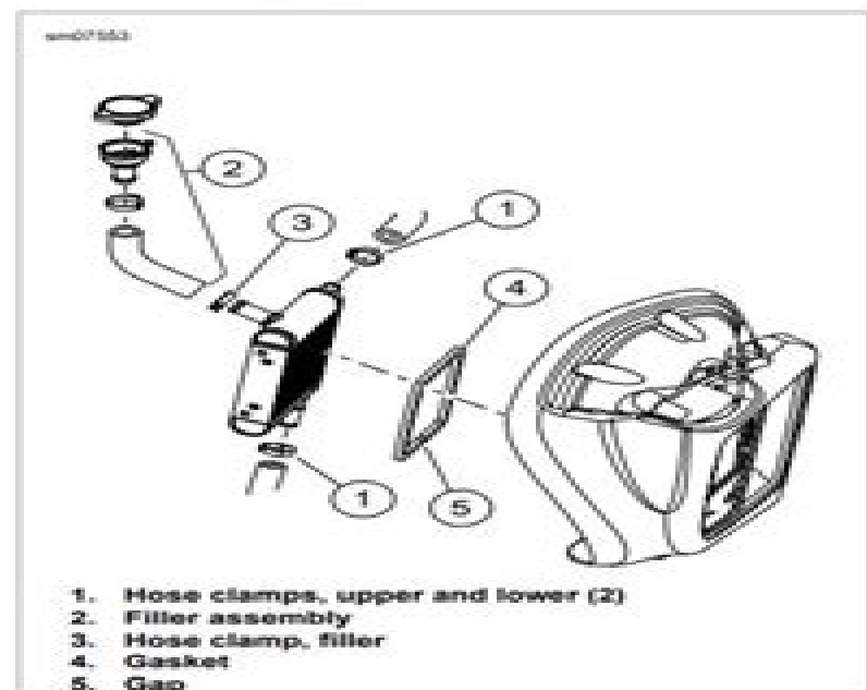
Figure B-10. Radiator
