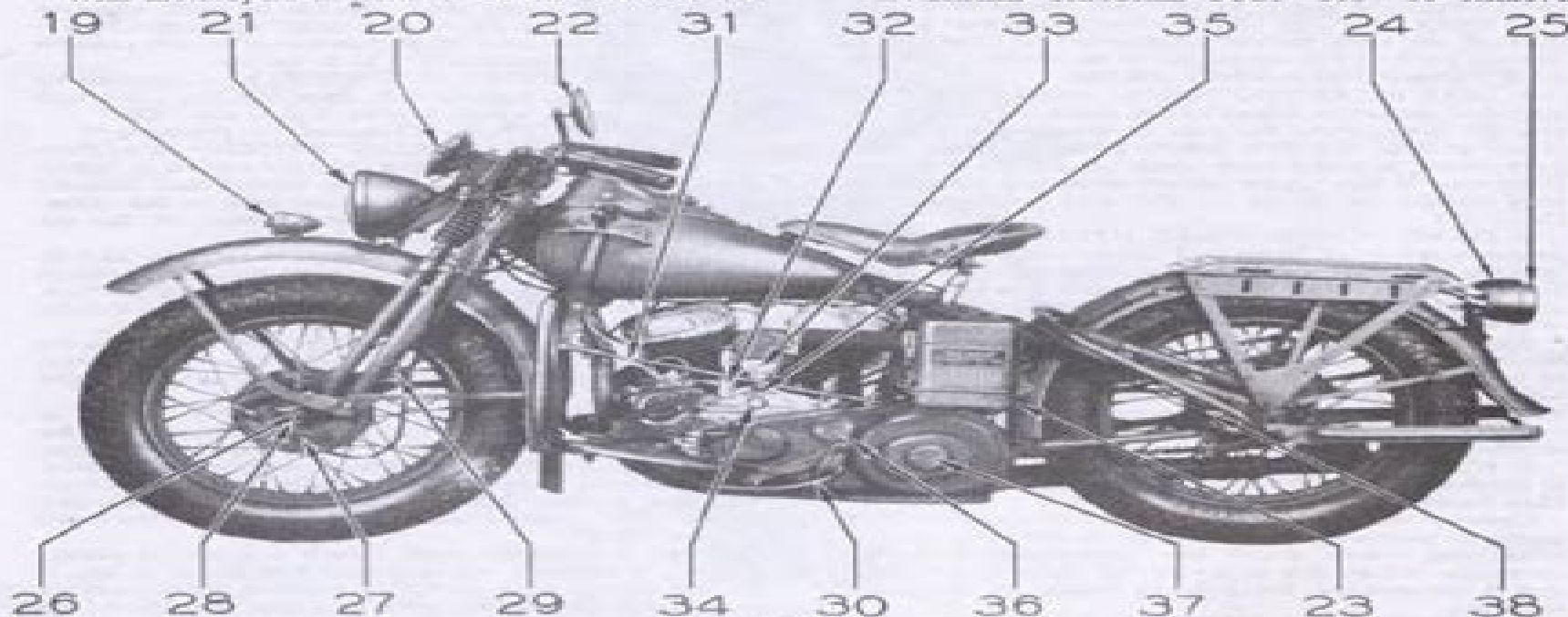
ILLUSTRATION 4 LEFT SIDE VIEW, DETAILS 19 TO 38
