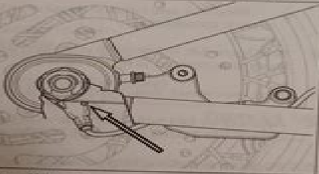
Figure 3-8. Rear Wheel Speed Sensor Orientation
