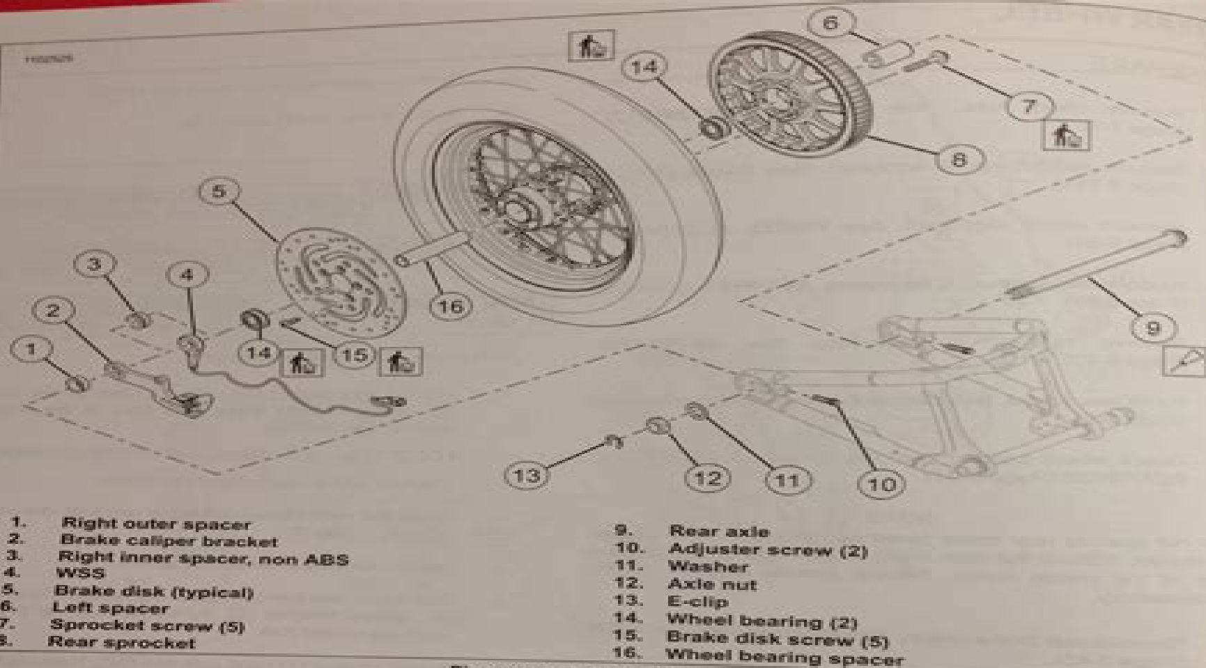
Figure 3-7. Rear Wheel
