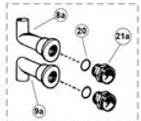
Original Side Mount Bulkhead Assembly (1995 and Prior)
