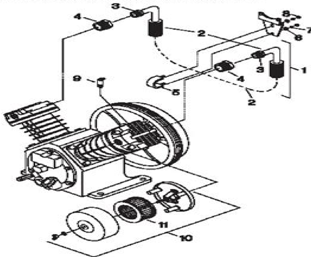
FIGURE 8. INTERCOOLER ASSEMBLY &amp; TUBING. (CLOCKWISE ROTATING UNIT SHOWN BELOW.)
