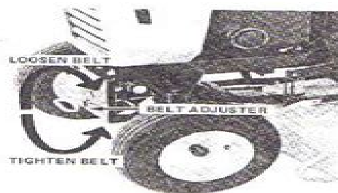
FIGURE 15 BELT ADJUSTMENT
