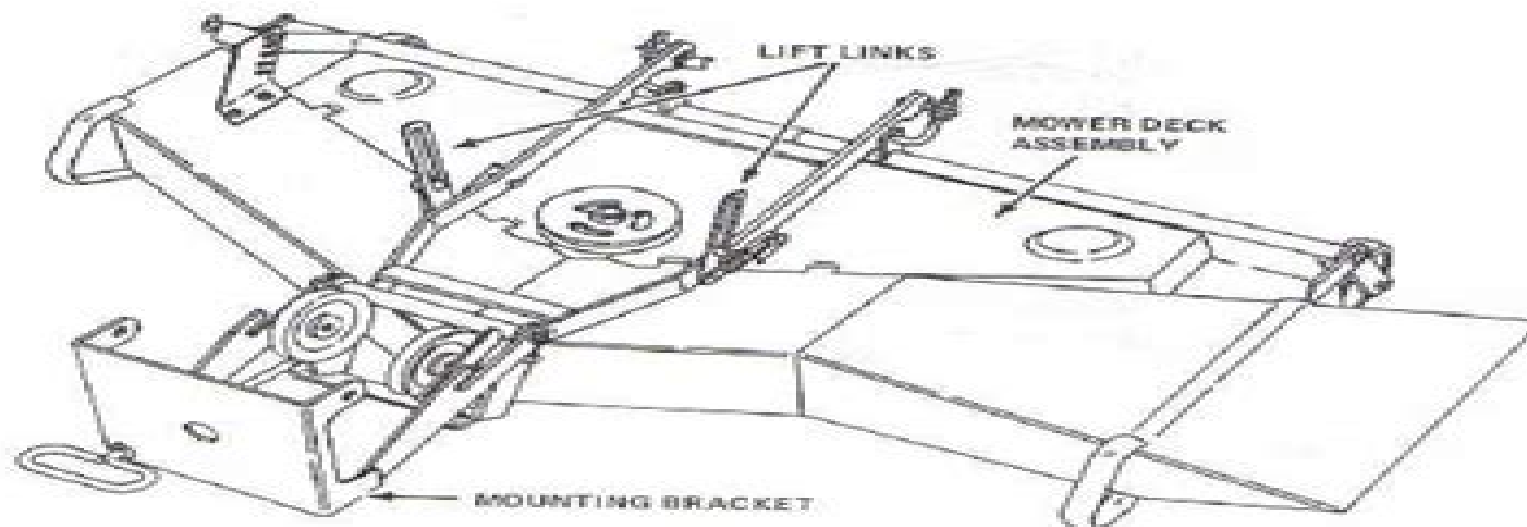
FIGURE 14 MODEL L44 ROTARY MOWER - ASSEMBLED
