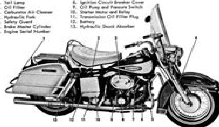
FIGURE 1. RIGHT SIDE VIEW
