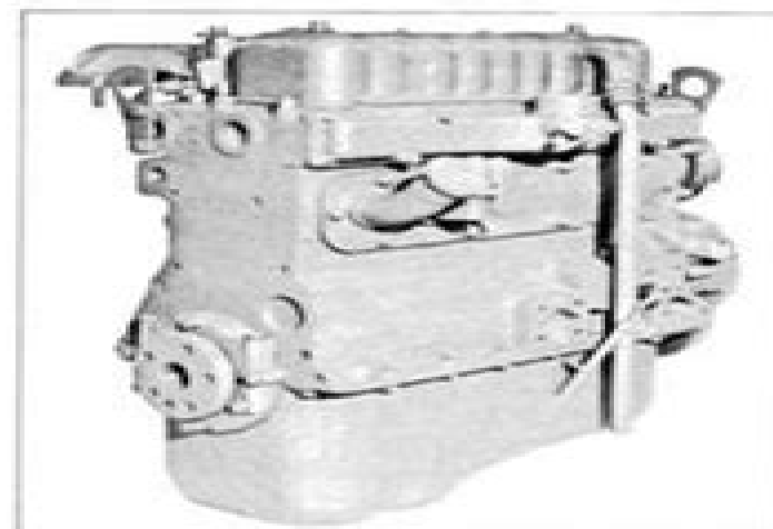
Fig. 2 - Rear Right-Hand View of A4.107 Engine
