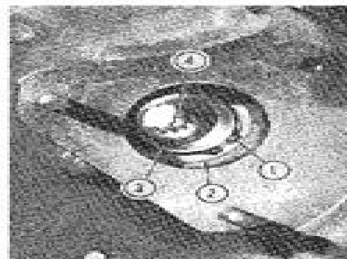
Fig. 22—Installed view of injection pump drive gear hub as seen from rear. Refer to Fig. 21 for parts identification.
