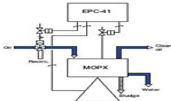
Fig. 2. Basic system-concept.
