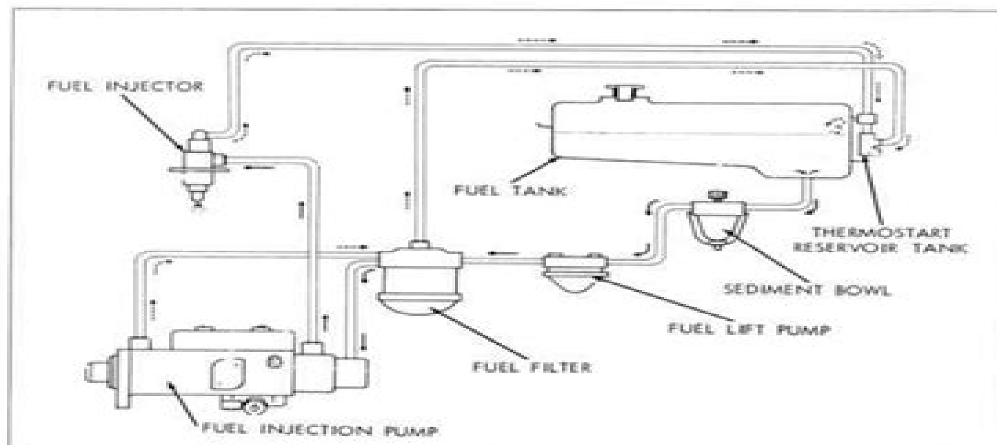
Fig. 1 - Fuel System of 4410P Engine
