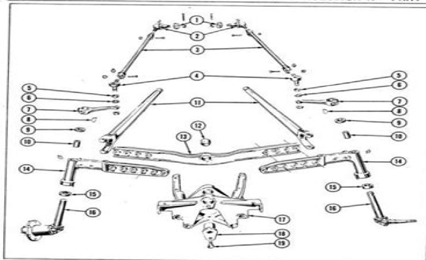
Fig. 1 - MF and TO 25 Front Axle Assembly Nomenclature
