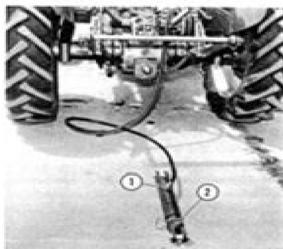
Fig. 14 - Hydraulically Retracting A Single-Acting Cylinder 1. Rod End Port 2. Breather
