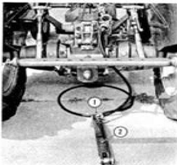
Fig. 13 - Hydraulically Extending A Single-Acting Cylinder 1. Piston End Port 2. Breather
