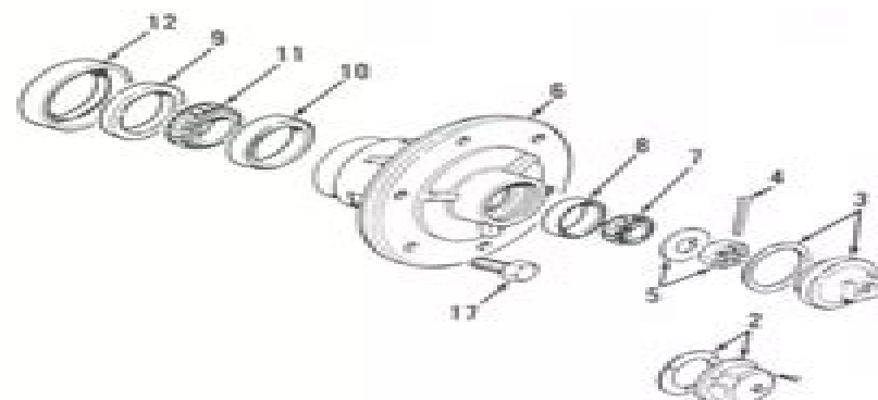
Fig. 4—Exploded view of wheel hub typical of two-wheel-drive models.
