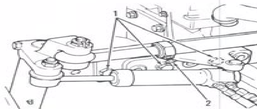
Fig. 5—View of axle left end typical of 362 model. Track adjusting screw and locknut (2) and cylinder bracket and axle extension screws (1) must be properly installed and tightened.
