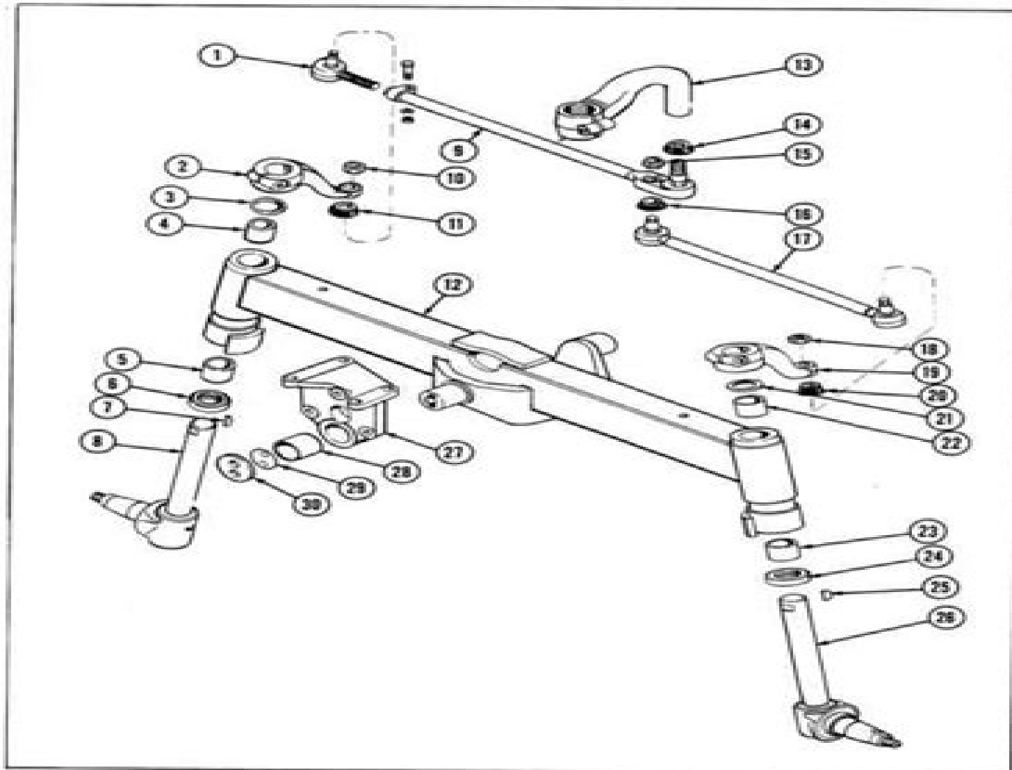
Fig. 3 - MF 65 Utility Front Axle Assembly Nomenclature.
