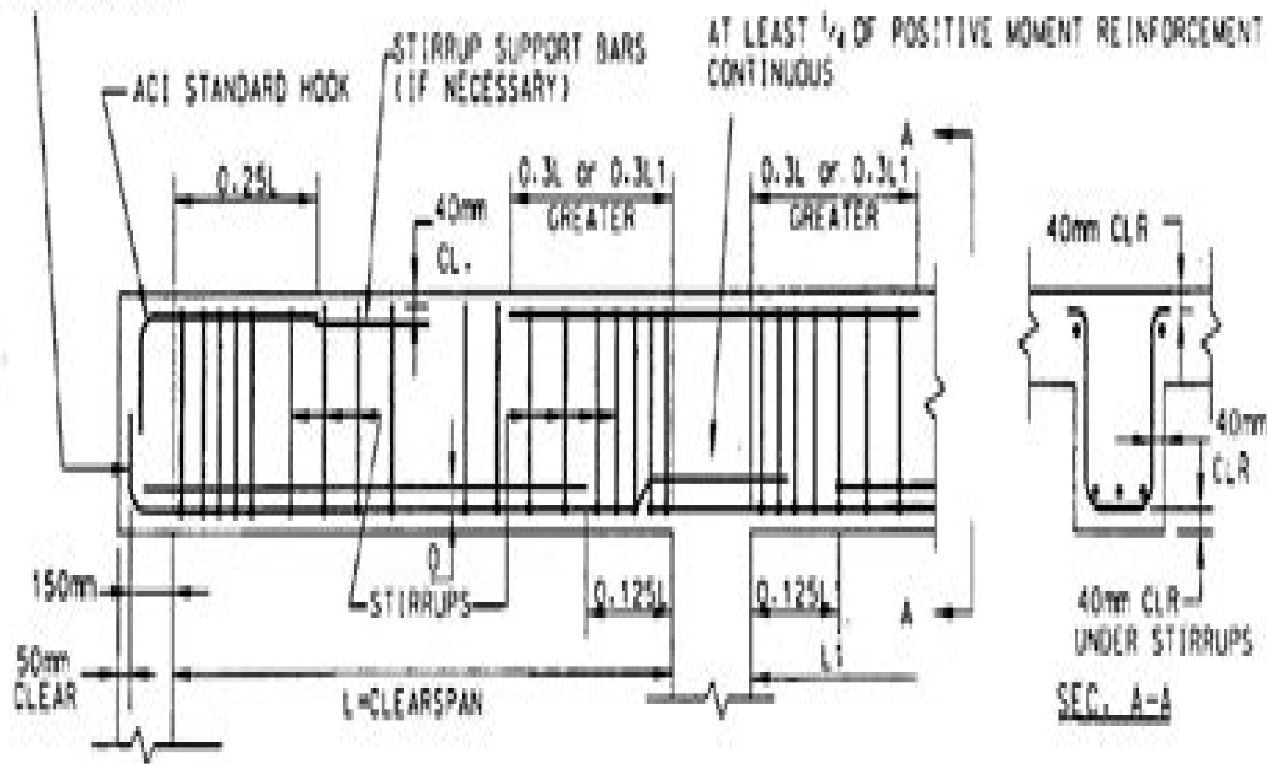
NON-PERIMETER BEAM WITH OPEN STIRRUPS
