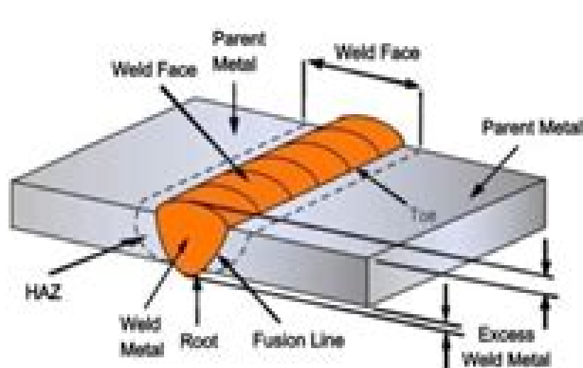
Butt joint
