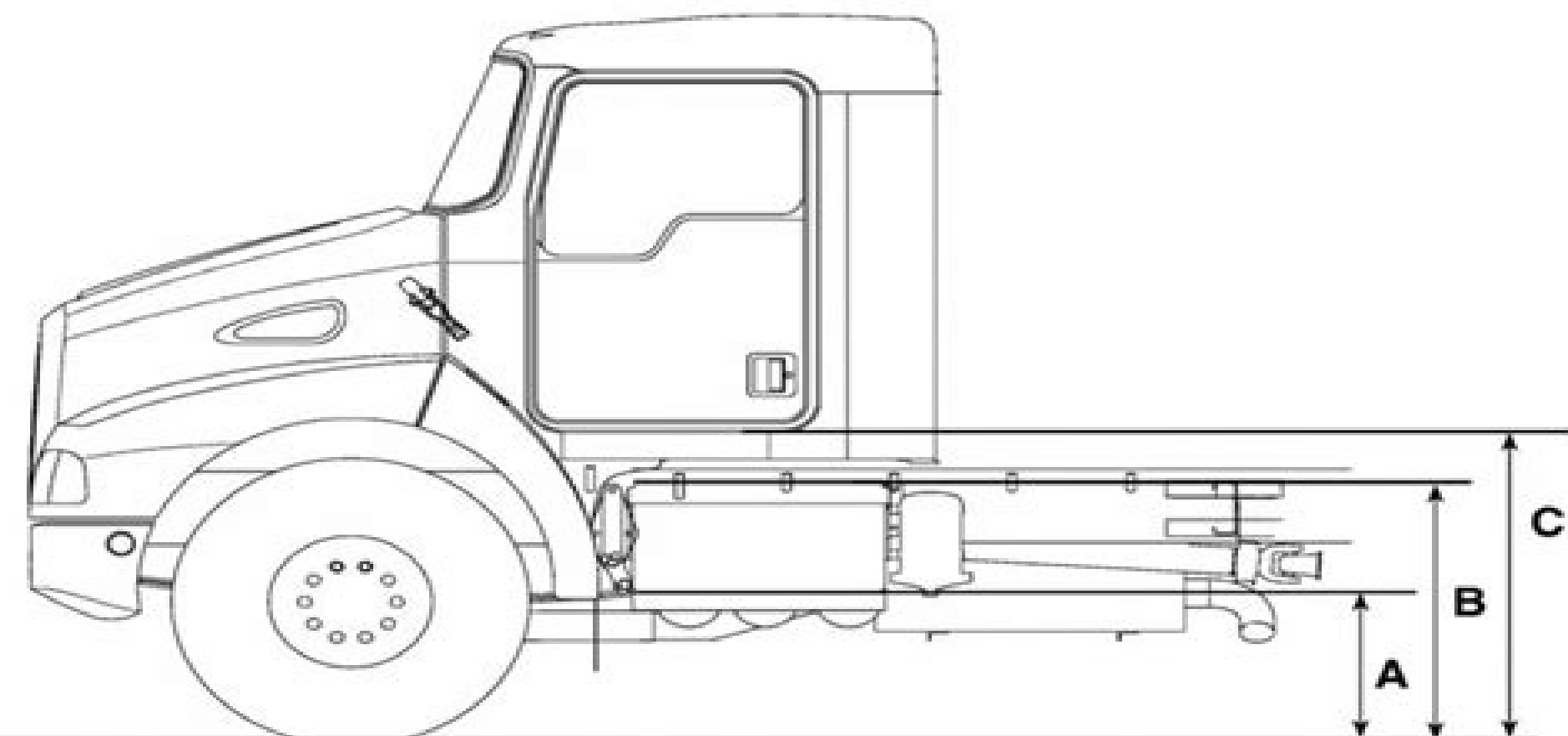
T300 Battery Box Step and Cab Floor: Side View, Left Side [inches (mm)].
