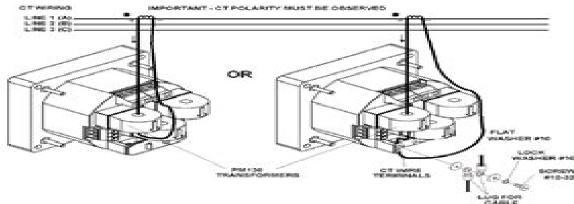
Figure 2-8 Current Input Connection
