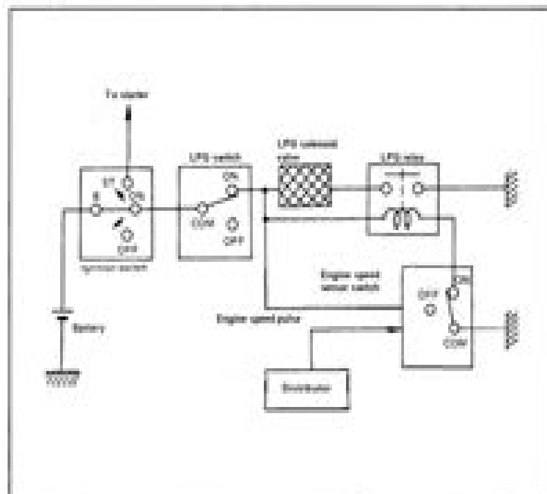
Wiring Diagram (When Engine is Operated)
