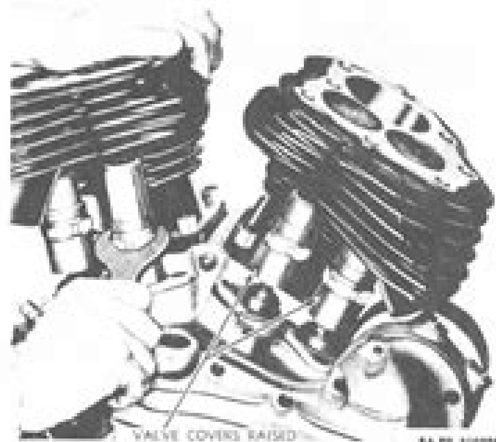
Figure 3—Freeing Valve Covers with Wrench (41-W-2617)
