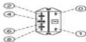
Relay contactor port no. assignment
