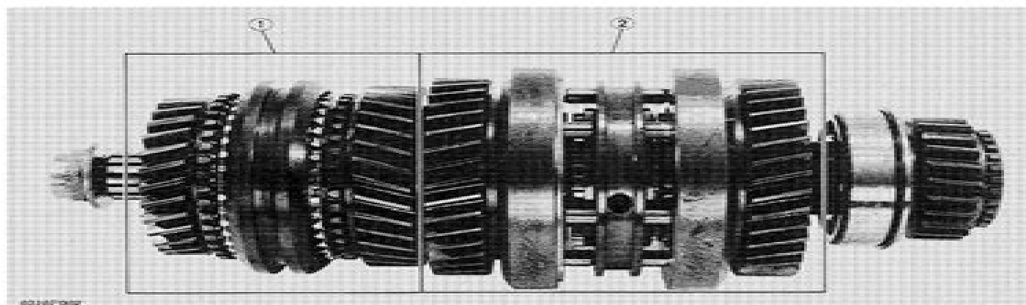
(1) Block-type Synchromesh (Main speed change 2nd-3rd speed)
