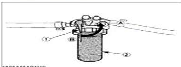
TABAAAAAP1310C (1) Fuel filter lever (2) Fuel filter pot
