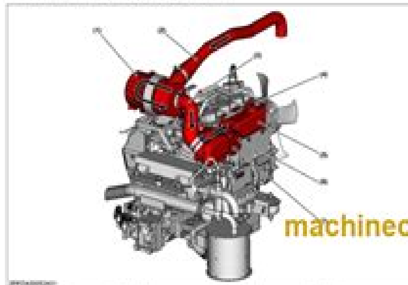
MECHANISM (1) Engine air cleaner (2) Intake duct (3) Intake manifold (4) Throttle body (5) Engine (6) MAF sensor
