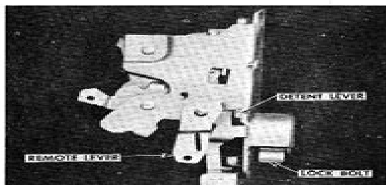
Fig. 30—Rotary Lock Parts
