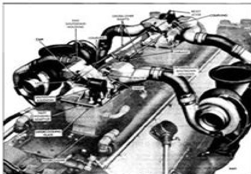
Fig. 3. Interconnected Engine Air Shutdown Housing Assembly
