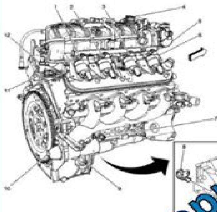
Fig. 6: Right Side of the Engine Courtesy of GENERAL MOTORS CORP.
