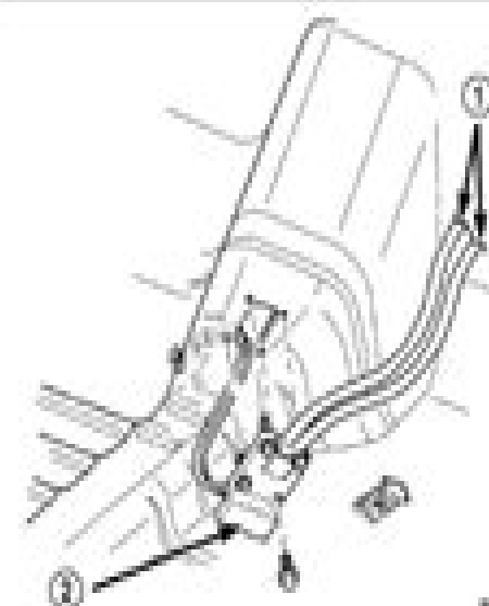
Fig. 153 Shift Cable Assembly at Floor Pan
