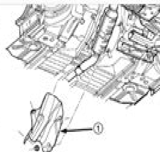
Fig. 152 Converter Heat Shield Removal/Installation 1 - CONVERTER HEAT SHIELD
