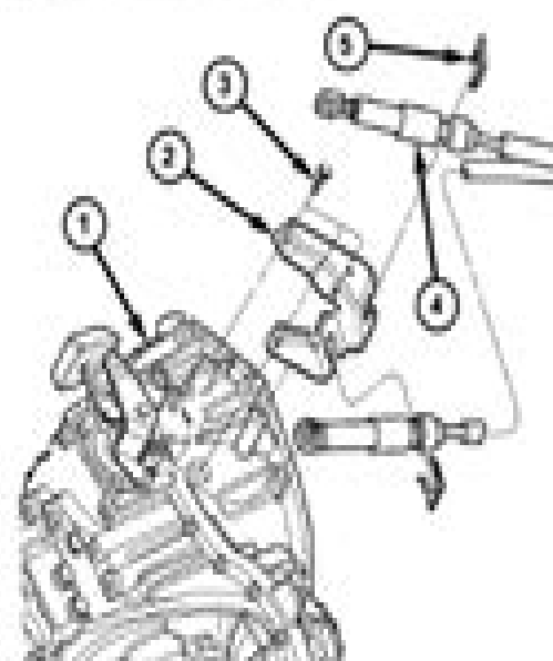
Fig. 151 Gear Shift Cables and Bracket at Transaxle
