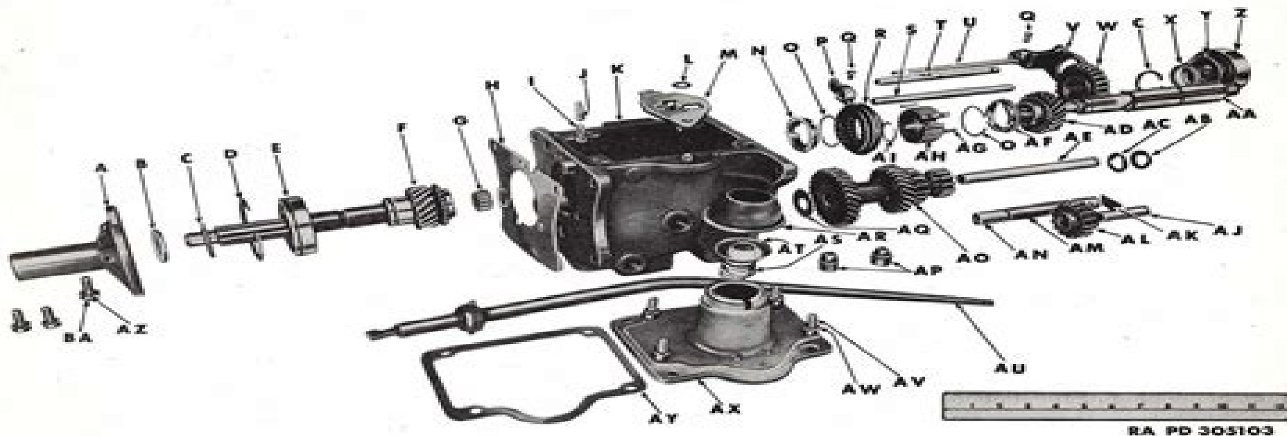
FIGURE 07-1—TRANSMISSION ASSEMBLY
