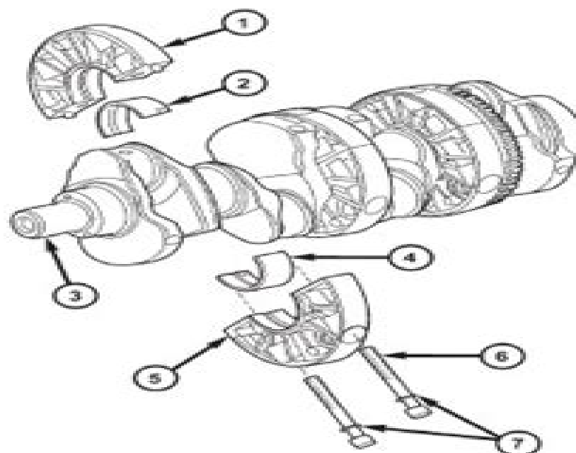
Fig. 34 CRANKSHAFT ASSEMBLY
