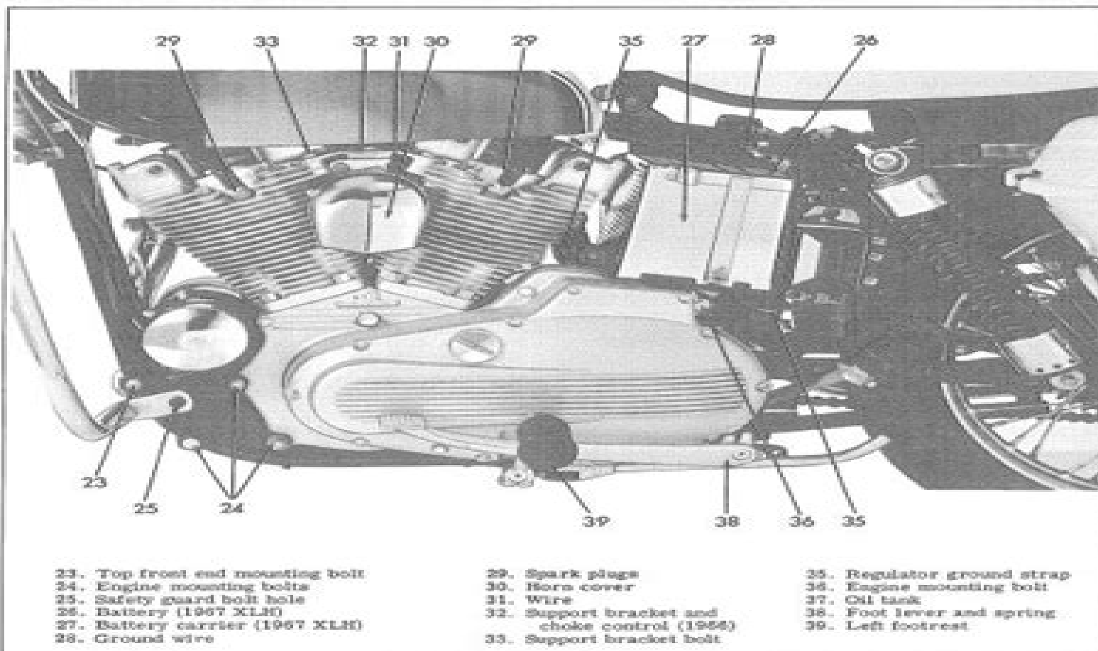
Figure 3A-8. Engine - Left Side View (1967 Model XLH Shown)
