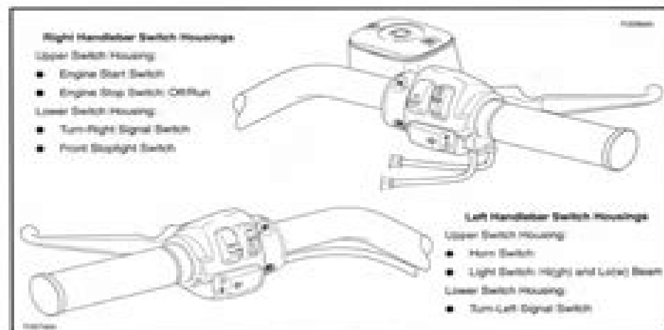
Figure 8-115. Road King Handlebar Switch Assemblies
