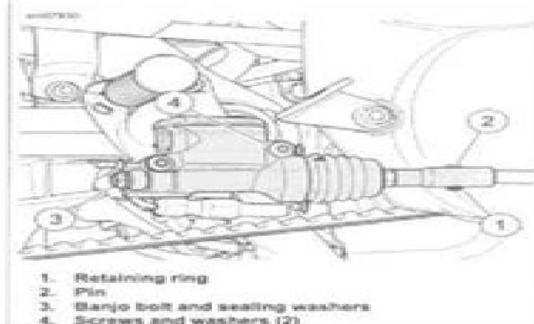
Figure 2-63. Rear Brake Master Cylinder
