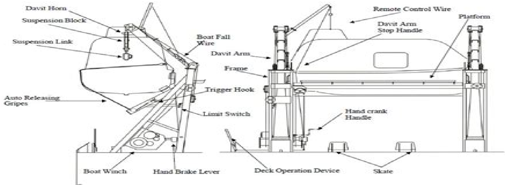
Fig. 1.1 Lifeboat davit arrangement
