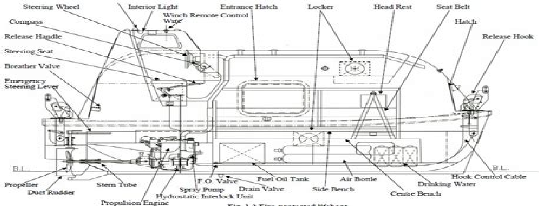
Fig. 1.2 Fire-protected lifeboat
