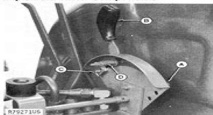
A—Height Stop B—Control Lever C—Depth Stop D—Friction Adjusting Screw
