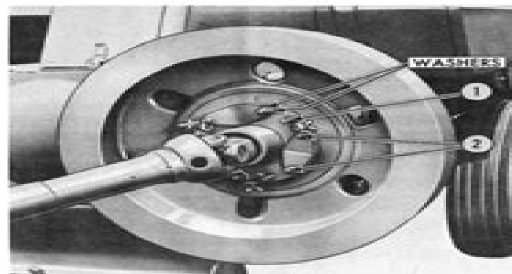
Figure 31 Friction Clutch
