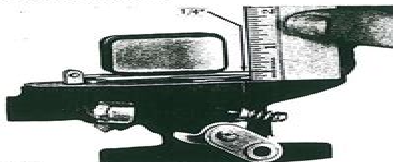
Fig. 90-25-18—Correct Float Position
