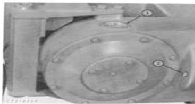
Fig. 11-Winch Oil Level
