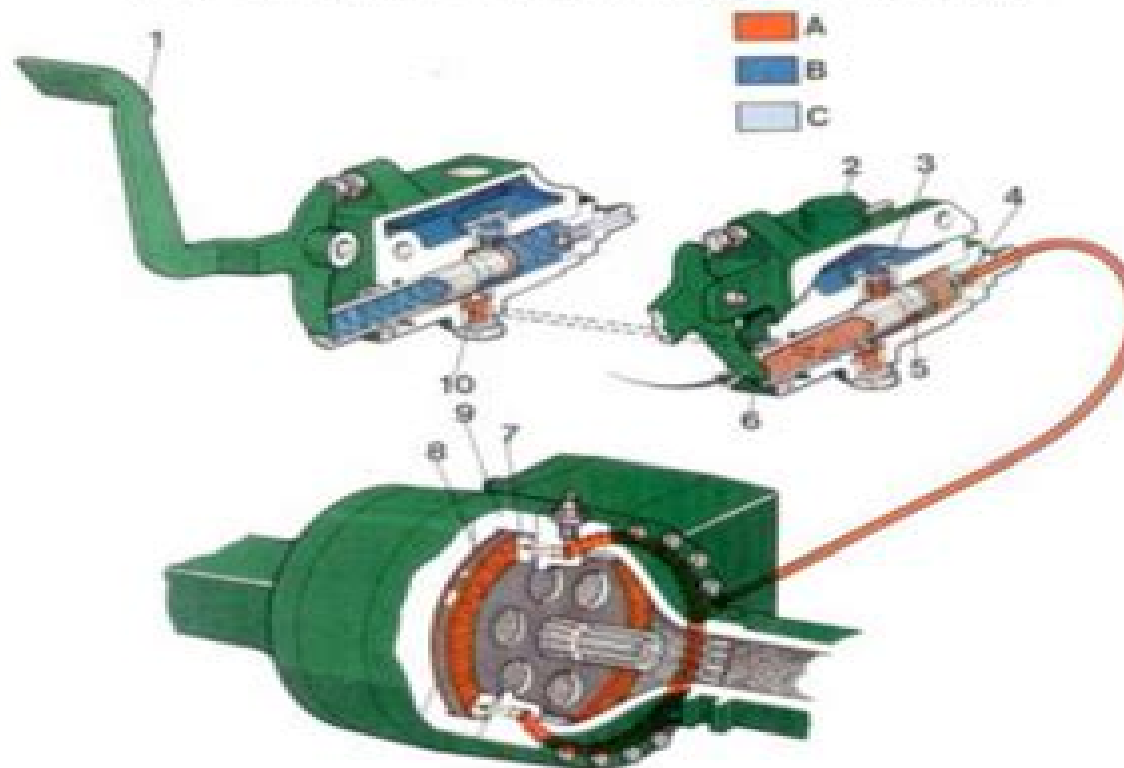
Fig. 3 - Oil Flow - Left Hand Brake Applied
